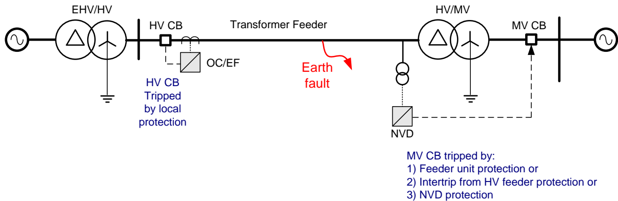
Figure 2-20 NVD Application
