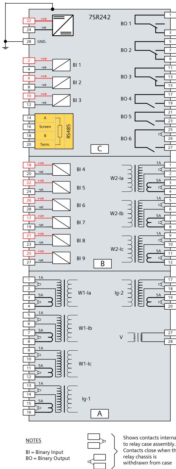
Figure 1-4 Connection Diagram: 7SR242 Relay
