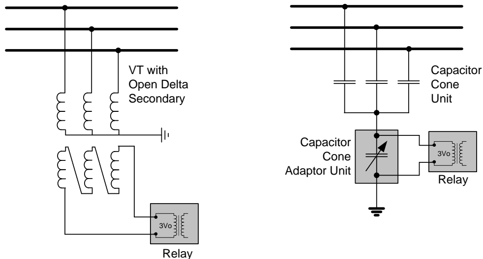
Figure 2-21 NVD Protection Connections
