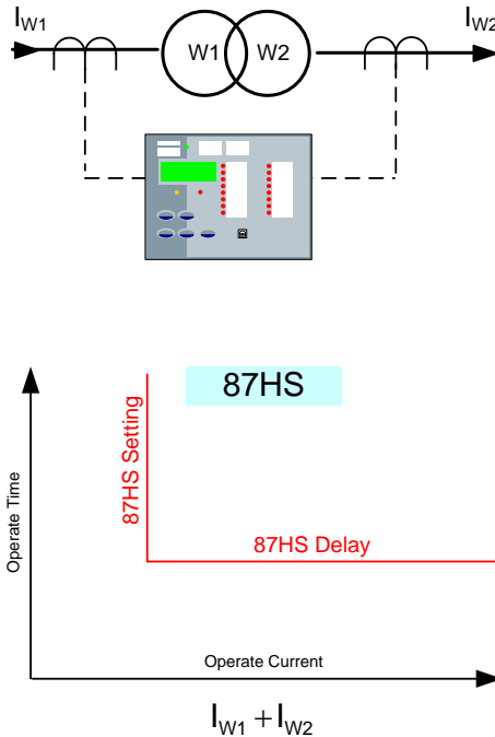
Fig. 2-3: Differential Highset Characteristic
