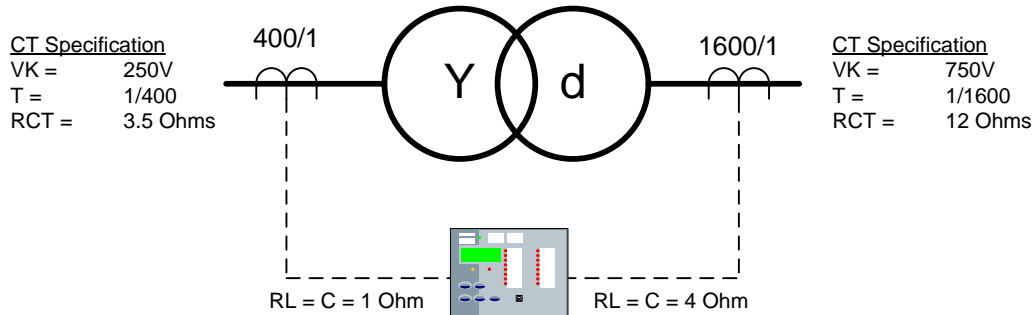
Figure 3-1 CT Requirements
