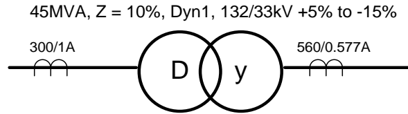
Figure 2-11 Relay Replacement
