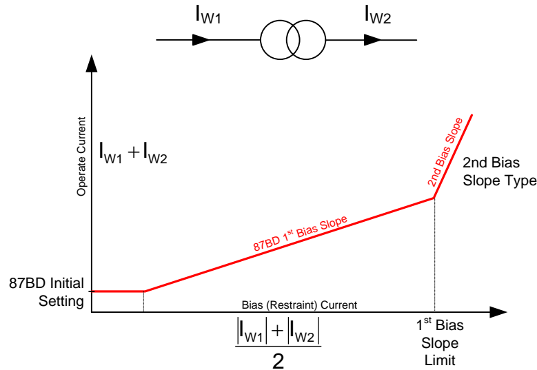
Figure 2-2: 87BD Characteristic
