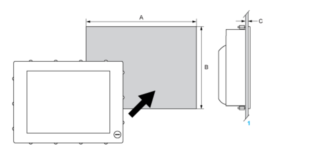
1 Installation panel
