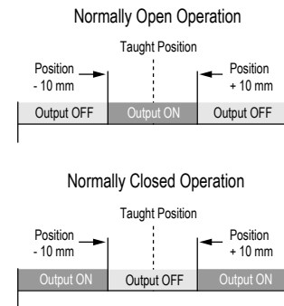
Using the Auto-Window feature for programming each output
