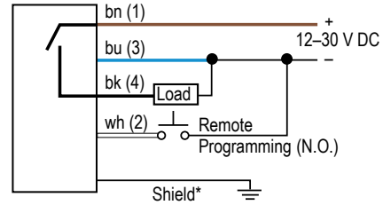
PNP (Sourcing) Output Models
