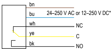
Q45VR3 sensors with attached cable
