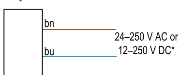
Q453E Emitters with attached cable
