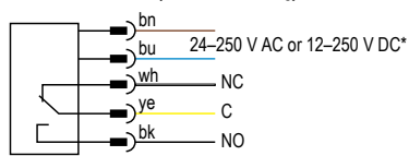
Q45VR3 sensors with quick-disconnect 5-pin Mini male (model suffix Q)
