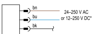
Q453EQ Emitters with quick-disconnect 3-pin Mini male
