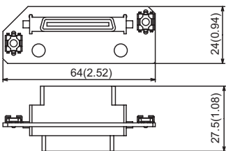
Extension interface relay board
