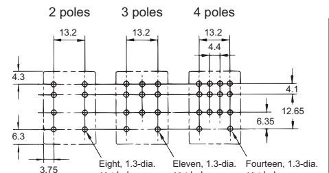
PCB Processing Dimensions (Bottom View)
