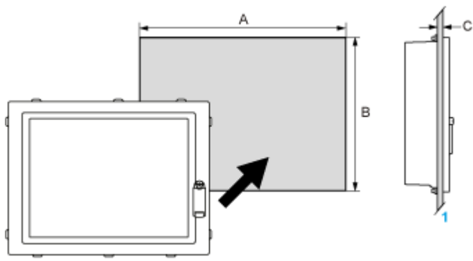
1 Installation panel
