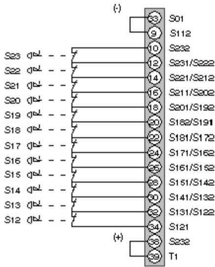
TELEFAST terminals
