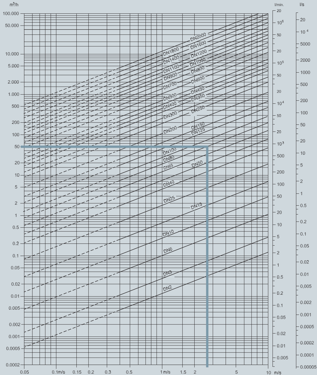
Sizing table (DN 2 ... DN 2000)
