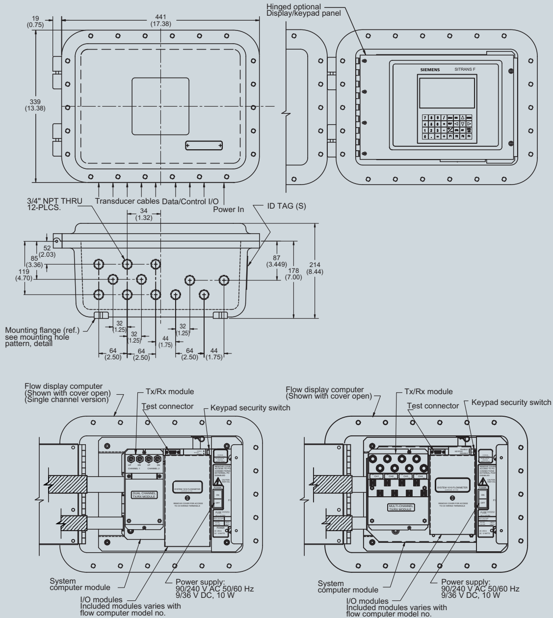
Single / Dual channel flowmeter
