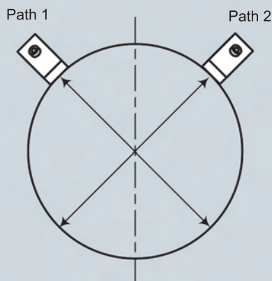
Dual Beam installation example
