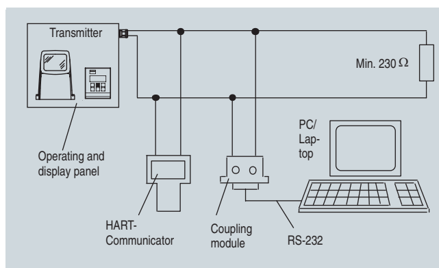
HART communication
