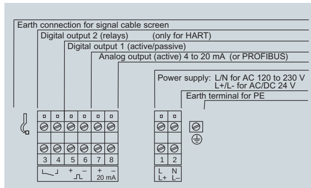
Electrical connection SITRANS FUS060
