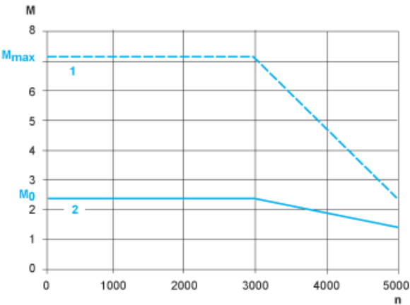
Servo Motor with LXM23•U07M3X Servo Drive
