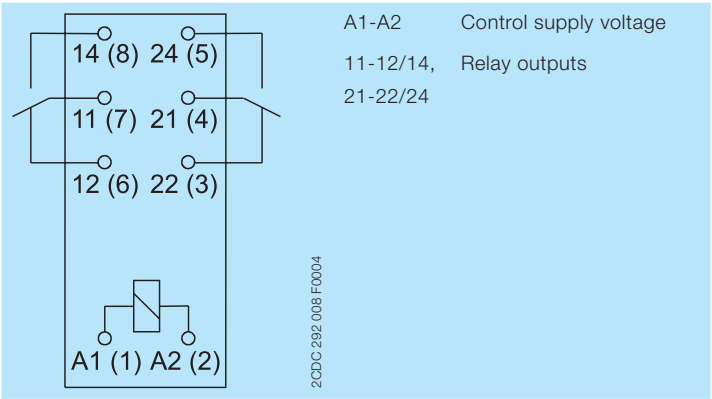
Connection diagram
