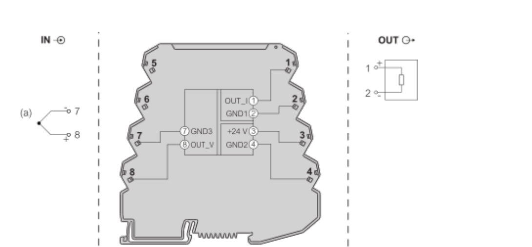
(a) : Thermocouple
