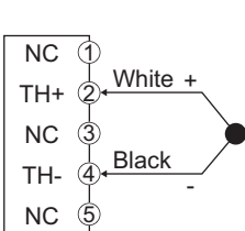
Thermocouple (TC)
