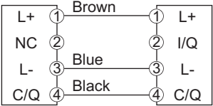
IO-Link master
