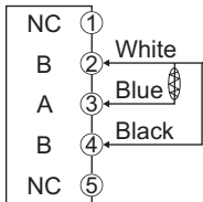
Resistance Temperature Detector (Pt)
