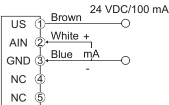
Analog input (I)
