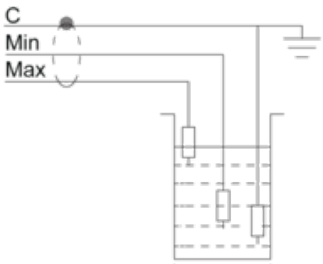
Wiring Diagram
