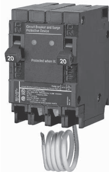
Circuit Breaker and Surge Protective Device (SPD)
