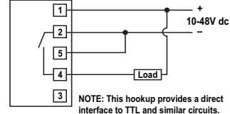
Alternative Low Saturation Sinking (NPN) Hookup
