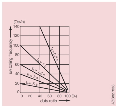
Motor starting time
