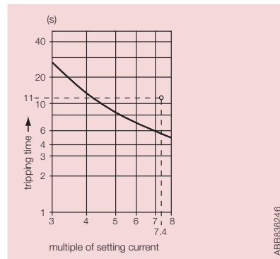
Tripping curve, starting from cold state
