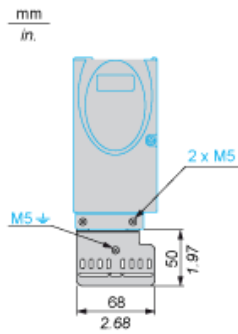
EMC mounting plate (included)
