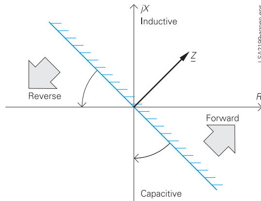
Fig. 5/81 Directional characteristic of the directional time-overcurrent protection
