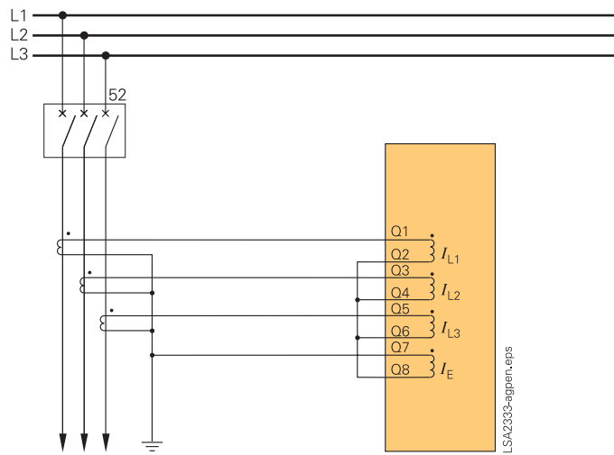
Fig. 5/92 Residual current circuit without directional element
