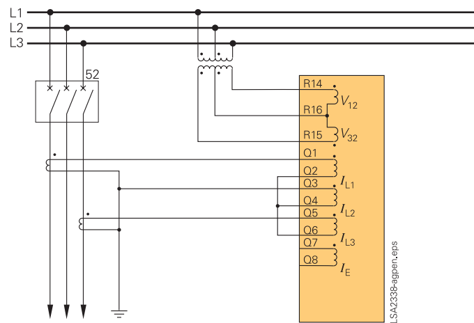
Fig. 5/97 Isolated-neutral or compensated networks
