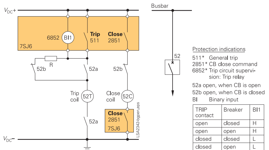
Fig. 5/101 Trip circuit supervision with 1 binary input
