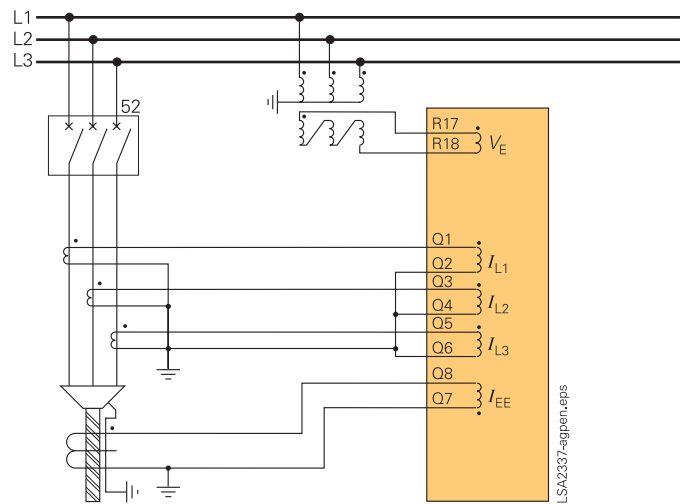
Fig. 5/96 Sensitive directional earth-fault detection
