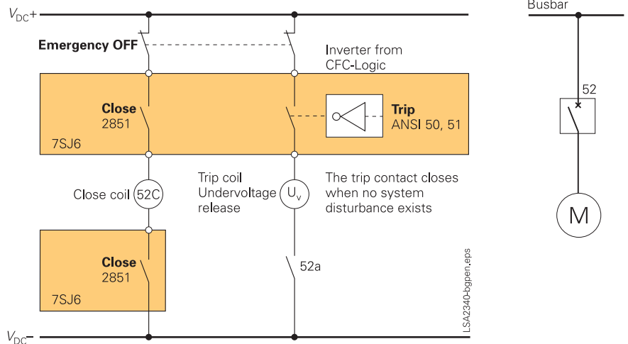
Fig. 5/99 Undervoltage trip with locking contact (trip signal 50 is inverted)
