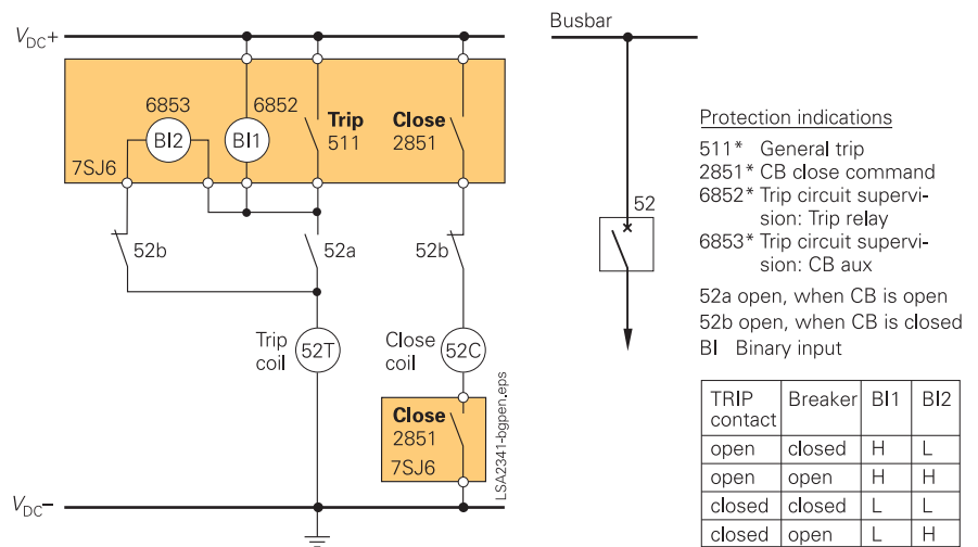
Fig. 5/100 Trip circuit supervision with 2 binary inputs
