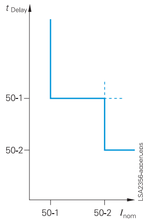
Fig. 5/79 Definite-time overcurrent protection
