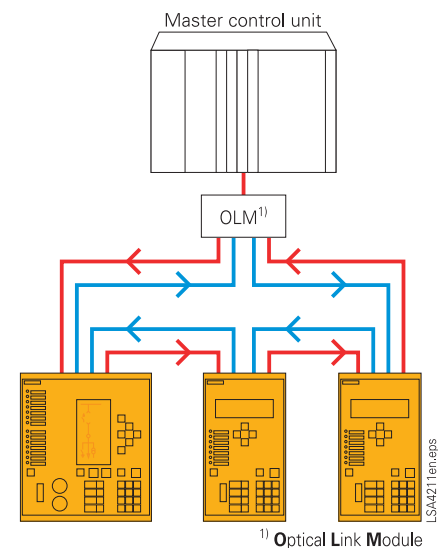
Fig. 5/88 PROFIBUS: Fiber-optic double ring circuit
