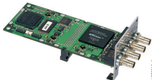
Fig. 5/91 Optical Ethernet communication module for IEC 61850 with integrated Ethernet-switch
