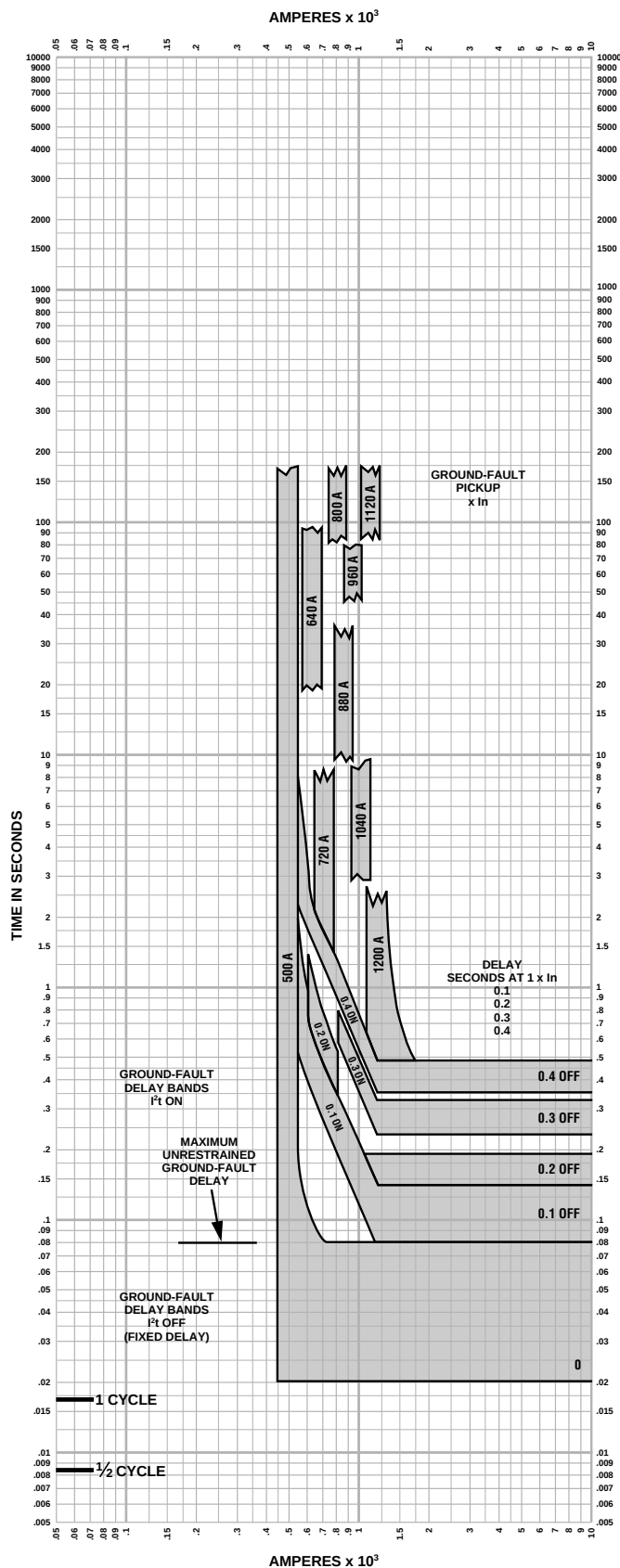
Figure 111 - MicroLogic 6.0 A/P/H Trip Units: I_n > 1200 \text{ A}
