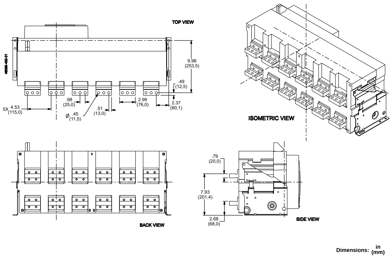
Figure 76 - 5000 A Rear Connected "T" Horizontal (RCTH)
