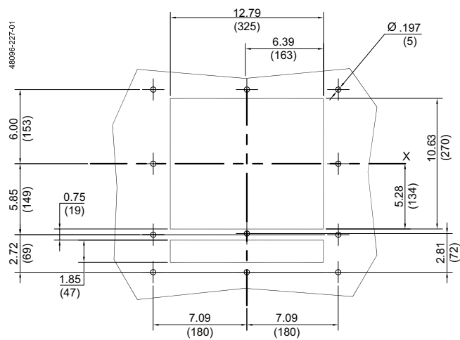
Figure 69 - Door Escutcheon Hole Pattern
