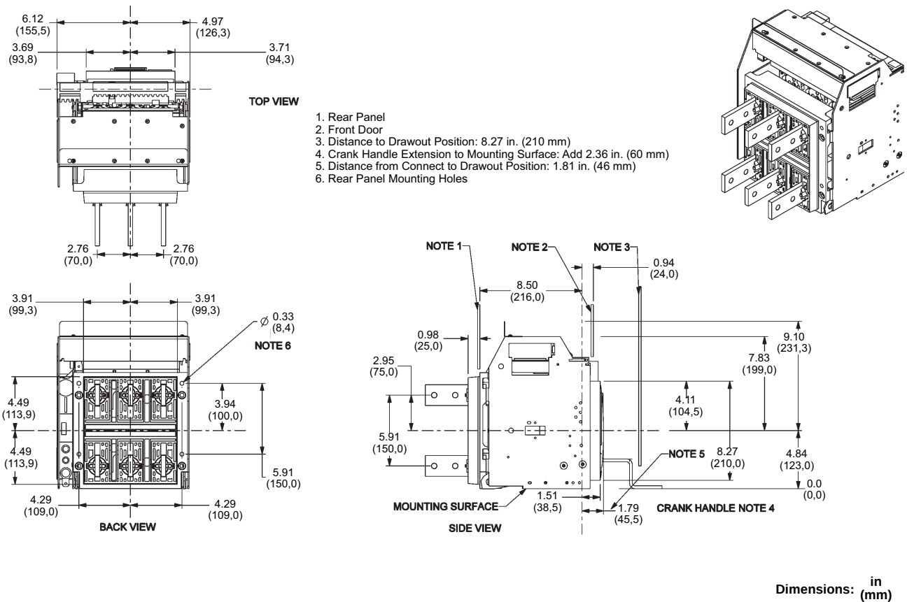
Figure 25 - 800–1600 A MasterPact NT Three-Pole Drawout—Master Drawing
