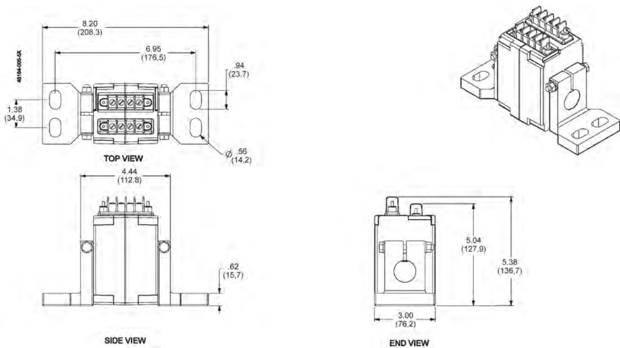
Figure 53 - 800–1600 A External Neutral Current Transformer
