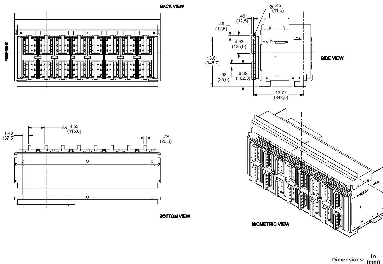
Figure 88 - 6300 A Rear Connected "T" Vertical (RCTV)
