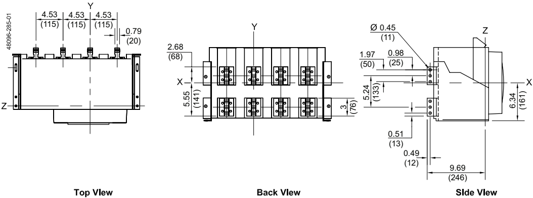
Figure 81 - 800–3200 A Rear Connected "T" Vertical (RCTV)
