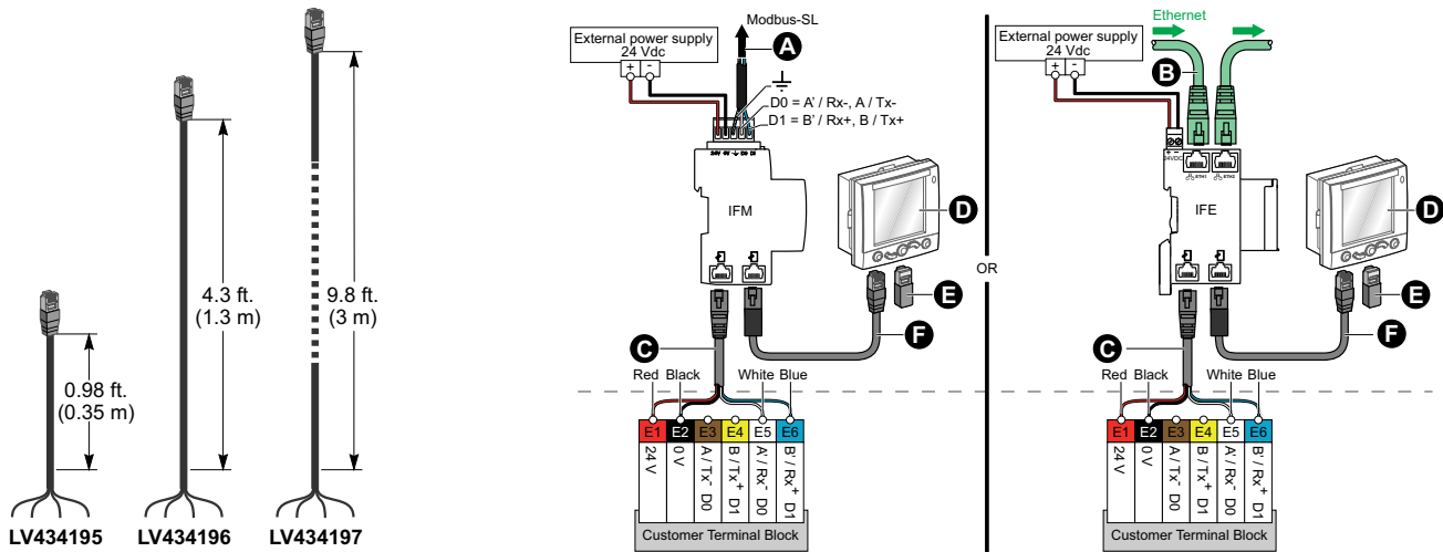
Circuit Breaker ULP Cord Connections
