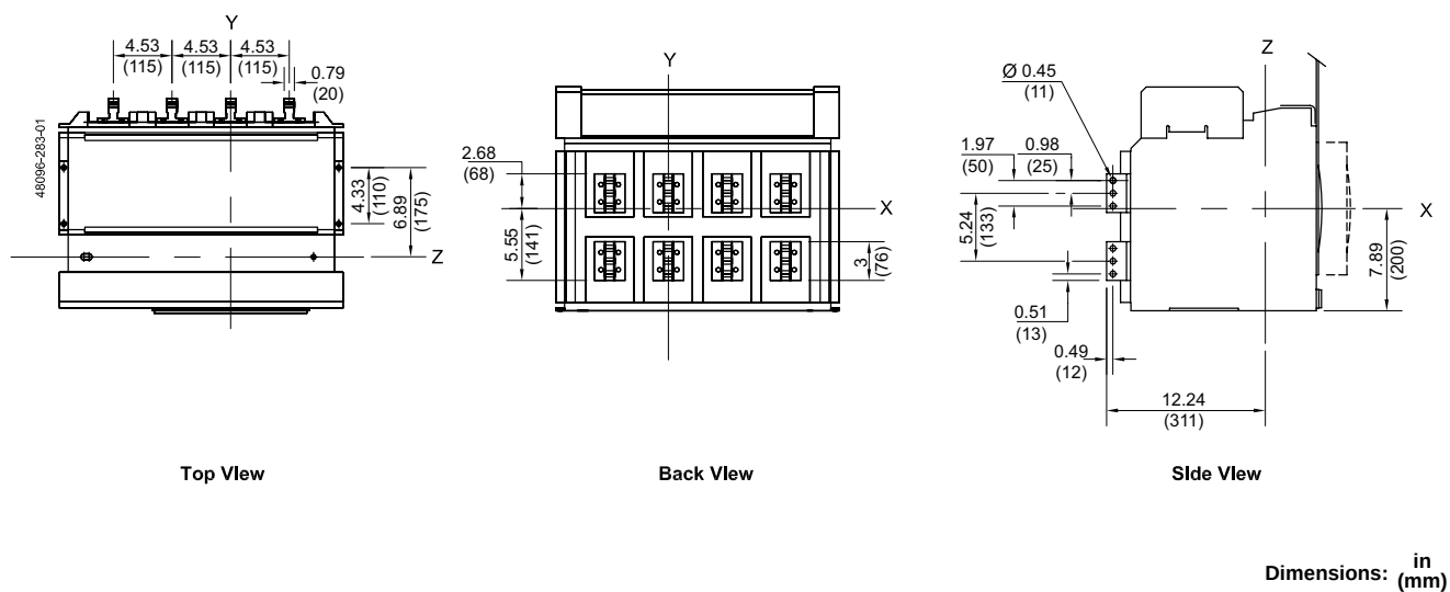
Figure 89 - 800–3200 A Rear Connected "T" Vertical (RCTV)
