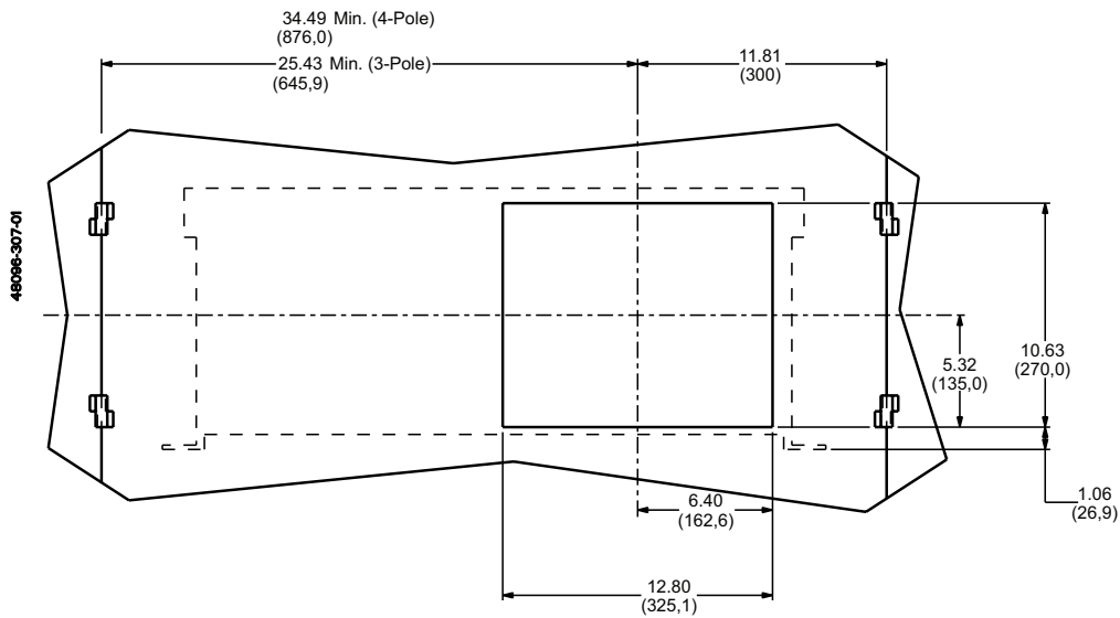
Figure 79 - 4000–6000 A Door Cutout
