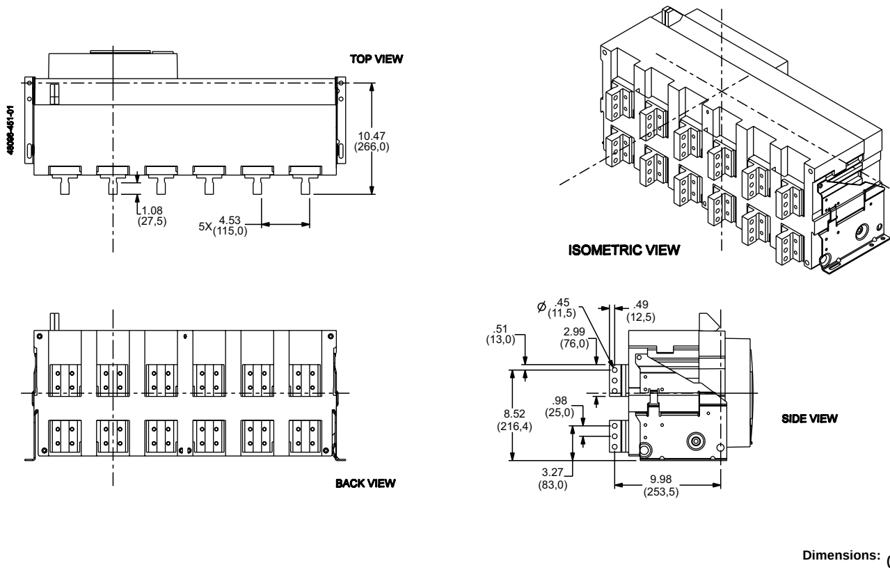
Figure 75 - 5000 A Rear Connected "T" Vertical (RCTV)
