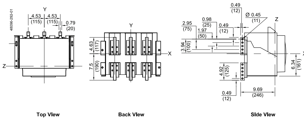
Figure 73 - 4000 A Rear Connected "T" Vertical (RCTV)
