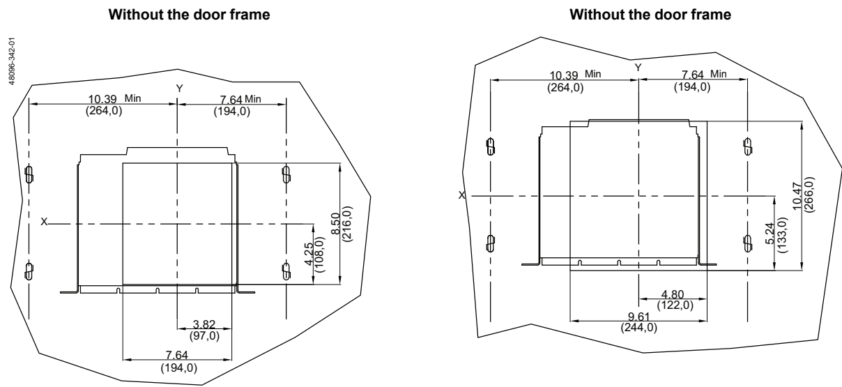
Figure 51 - 800–1200 A MasterPact NT 4P Fixed—Door Cutout Dimensions
