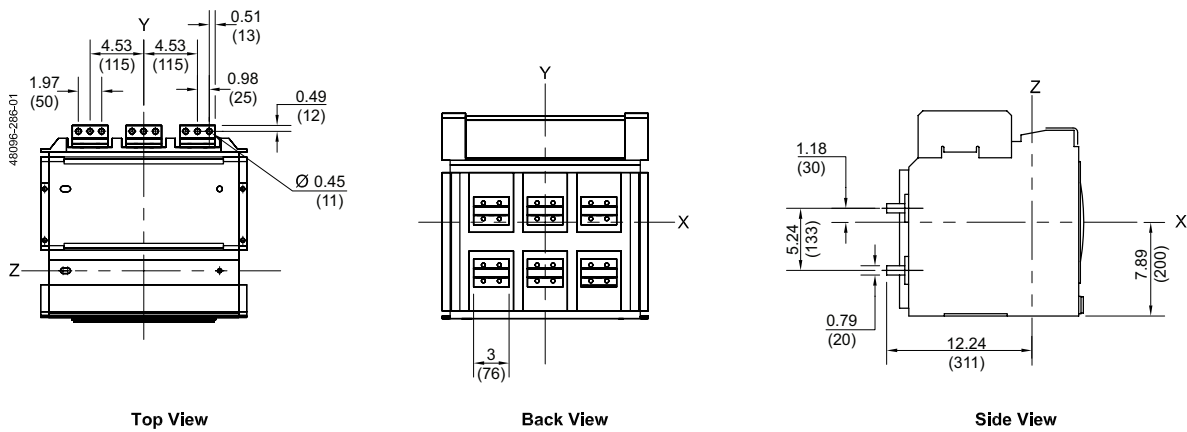
Figure 59 - 800–3200 A Rear Connected "T" Horizontal (RCTH)
