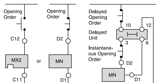
Figure 15 - Wire Diagram for the Remote Tripping Function
