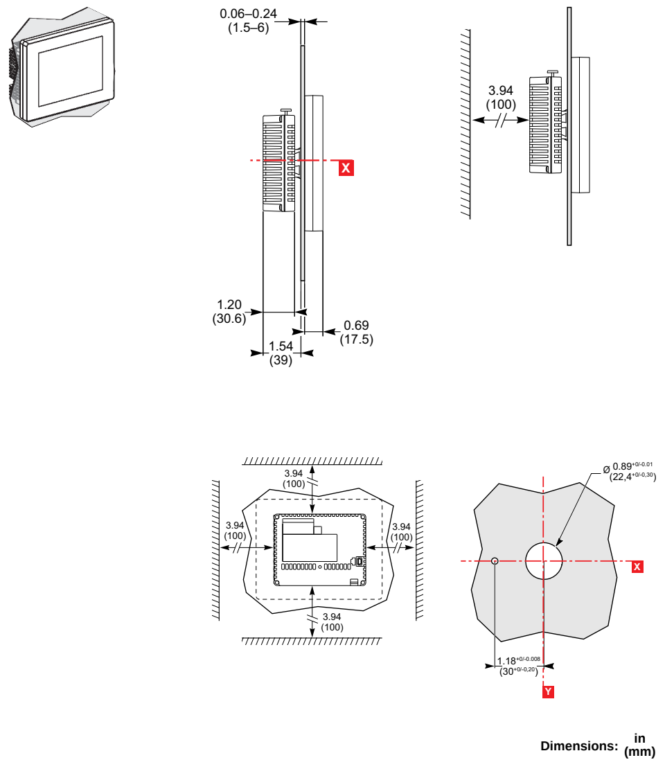
Figure 105 - FDM128 Switchboard Display Mounting on Panel
