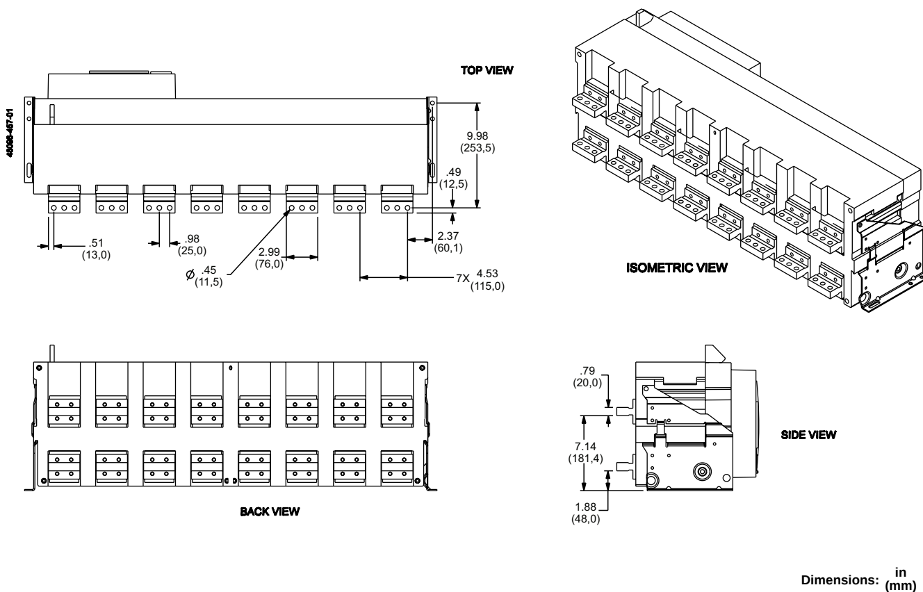
Figure 95 - 5000 A Rear Connected "T" Horizontal (RCTH)
