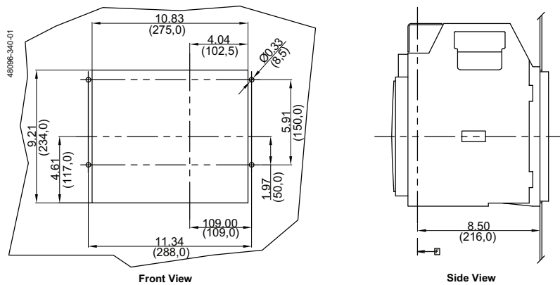
Figure 43 - 800–1200 A MasterPact NT 4P Drawout—Rear Cutout Dimensions
