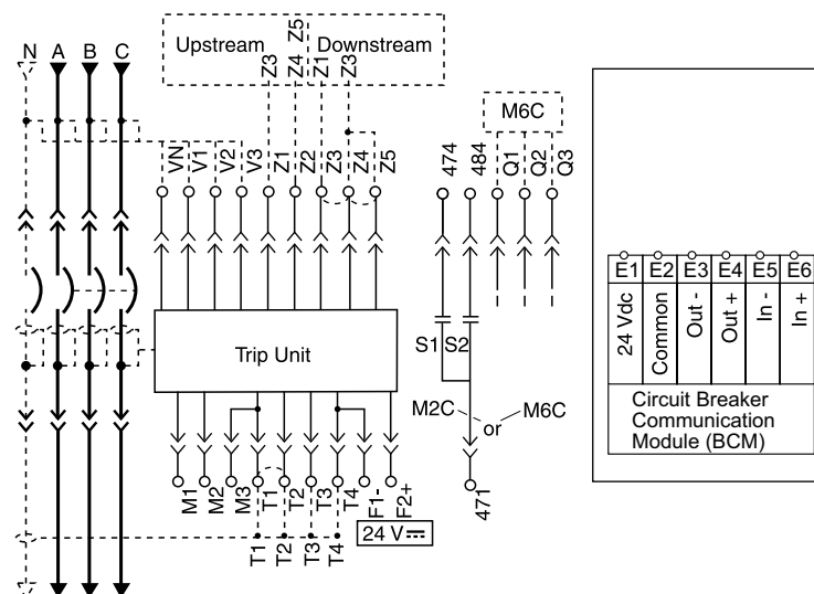
Figure 23 - Connection of the Communications Option
