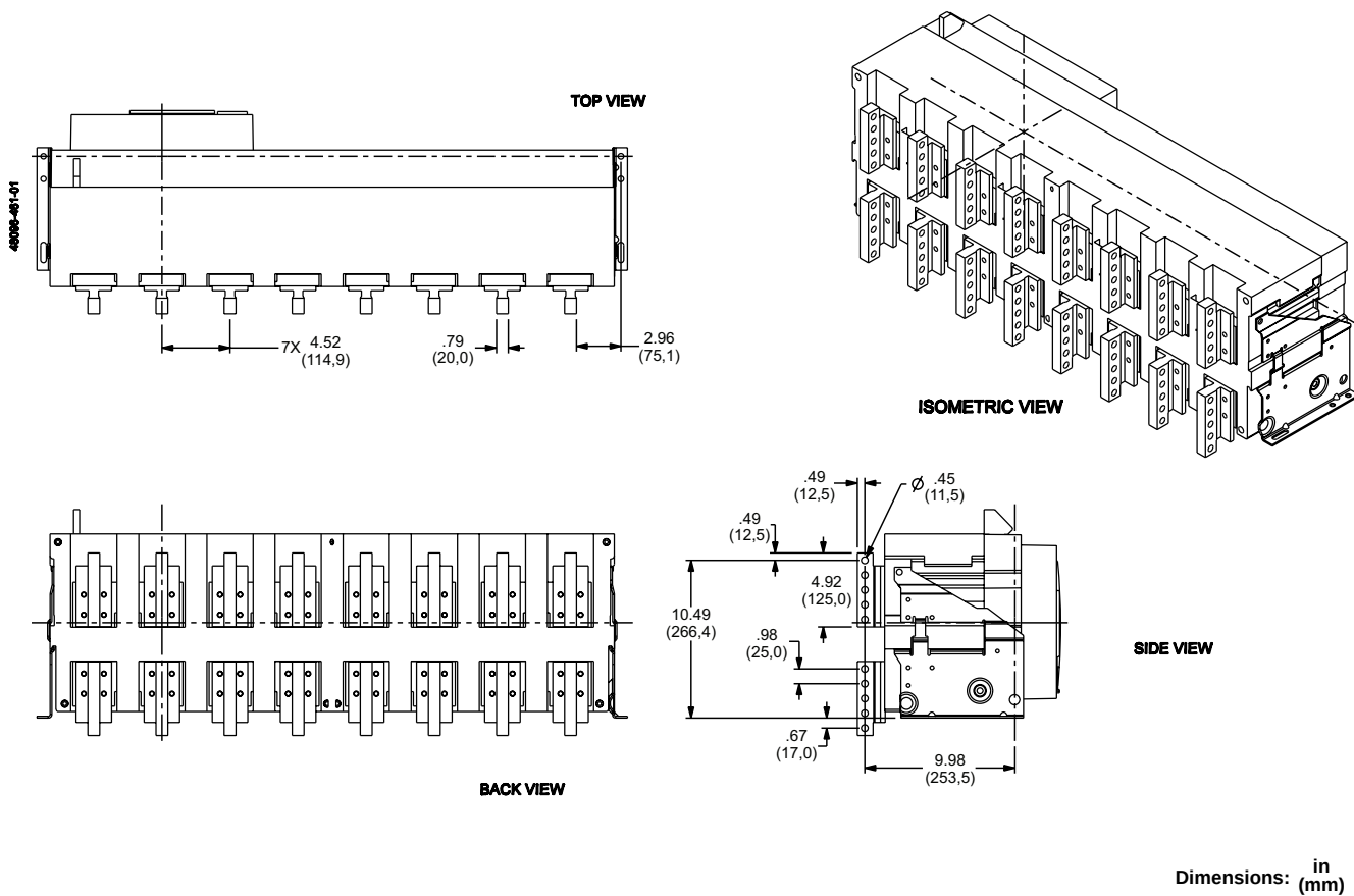
Figure 96 - 6300 Rear Connected "T" Vertical (RCTV)
