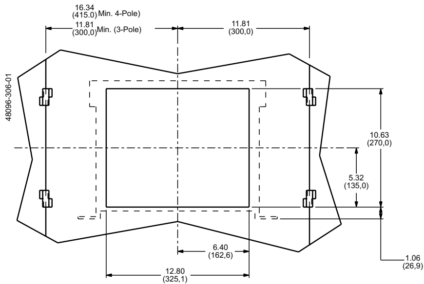
Figure 78 - 800–3200 A and 4000 A (W-Frame) Circuit Breaker Door Cutout
