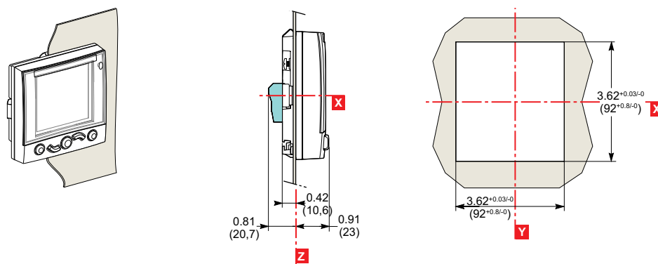
Figure 102 - FDM121 Switchboard Display Mounting Through Panel
