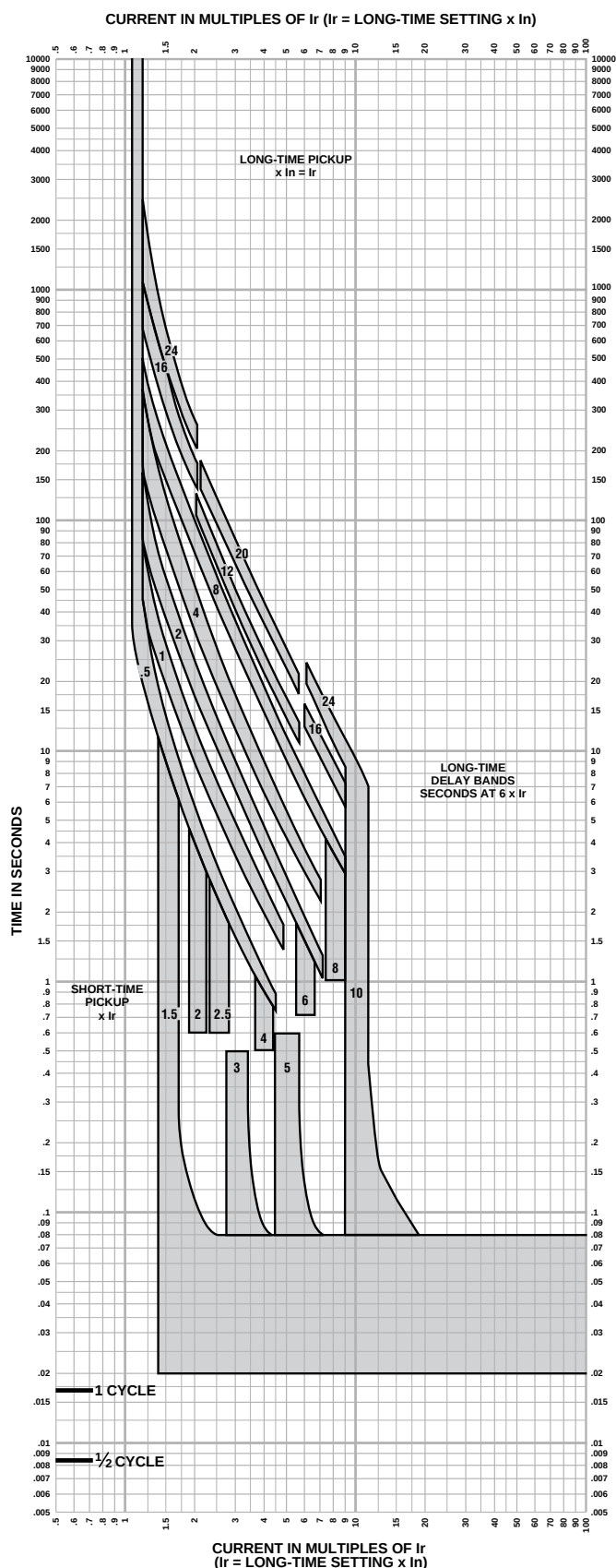
Figure 115 - MicroLogic 2.0A Trip Unit
