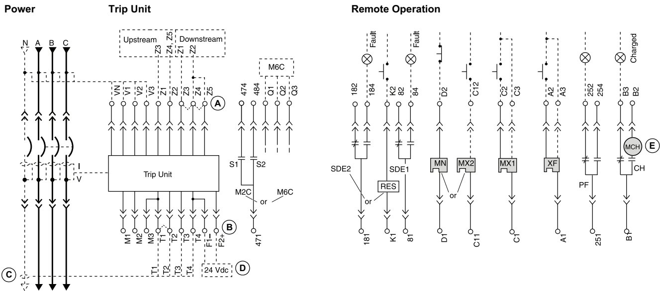
Figure 20 - Wiring Diagrams for MasterPact NW Circuit Breakers
