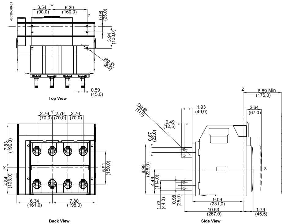
Figure 40 - 800–1600 A MasterPact NT 4P Drawout—RCTV Rear Connected “T” Vertical
