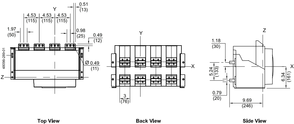
Figure 82 - 800–3200 A Rear Connected "T" Horizontal (RCTH)
