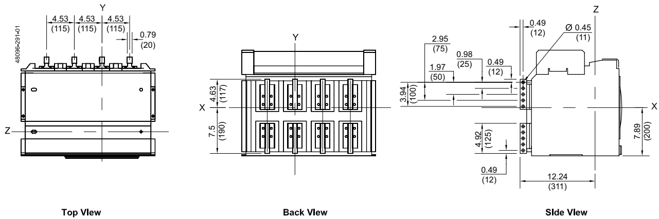
Figure 84 - 4000 A Rear Connected "T" Vertical (RCTV)
