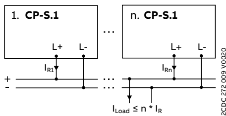
Parallel operation, increased power ( n \leq 3 )
