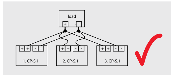
Correct wiring for increased power
