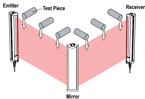
Figure 17. Trip Test with Corner Mirror
