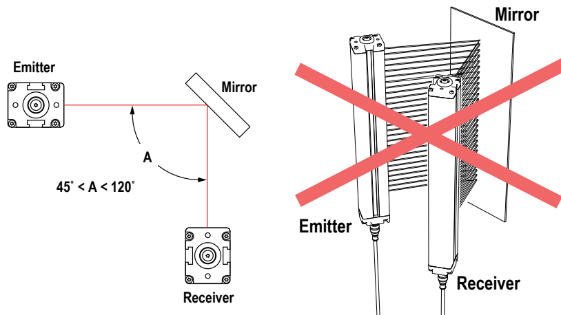
Figure 6. Using EZ-SCREEN Type 2 sensors in a retroreflective mode
