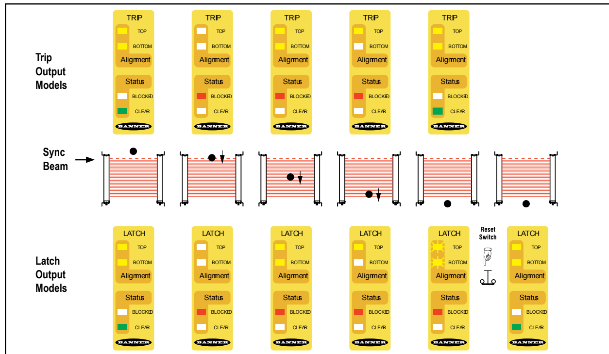
Figure 21. Status Indicator behavior during the trip test
