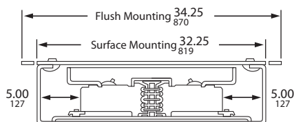
Typical Mounting of BD, BG, BJ, BK, FA, FH, HD, HG, HJ, HL, HR, JD, JG, JJ, JL, JR, QB, QD, QG, QJ
