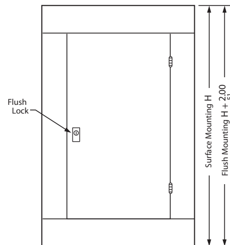
Typical 4-Piece Trim with Optional Door
