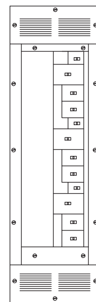
Typical 2-Piece Trim without Optional Door
