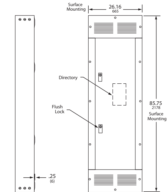
Typical 2-Piece Trim with Optional Door
