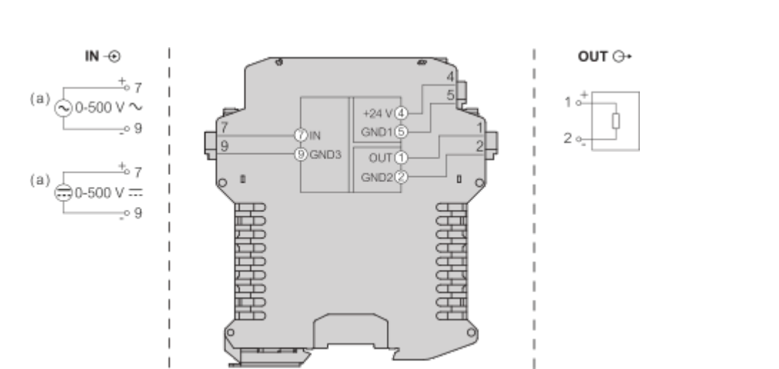
(a) : AC/DC Voltage Source
