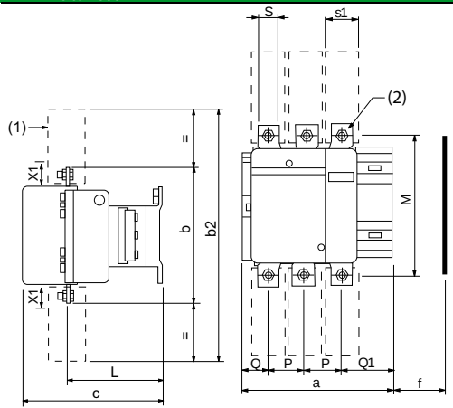
LC1F115 to F330
