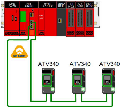
CIP Safety architecture
