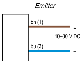
4-pin M8 male pinout
