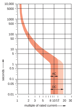
S204UP-K, 4 pole
