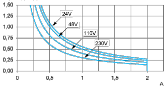
AC12 curves
