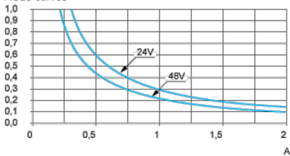
AC15 curves
