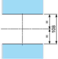
n circuit breakers GV7R side by side
