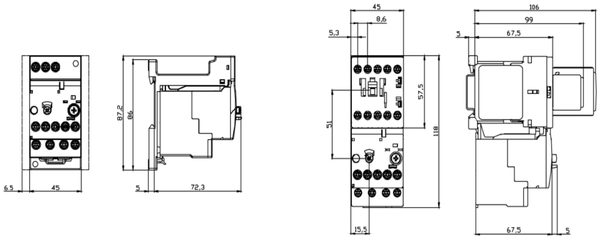
3RU7116 Mounting with Stand-alone adaptor
