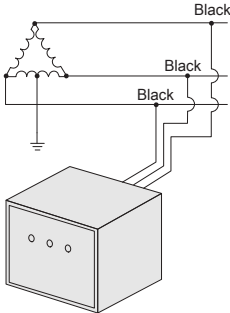
3-Phase, 4-Wire High-Leg Delta
