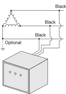
3-Phase, 3-Wire Delta
