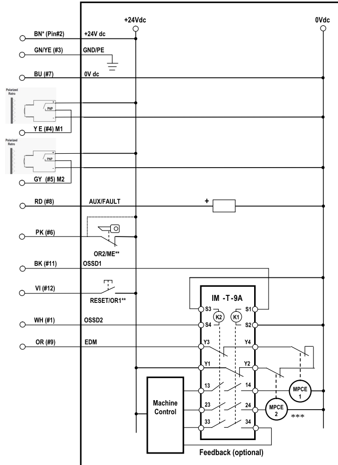
Figure 30. Generic wiring - Interface Module (1-CH EDM, manual reset, Override)
