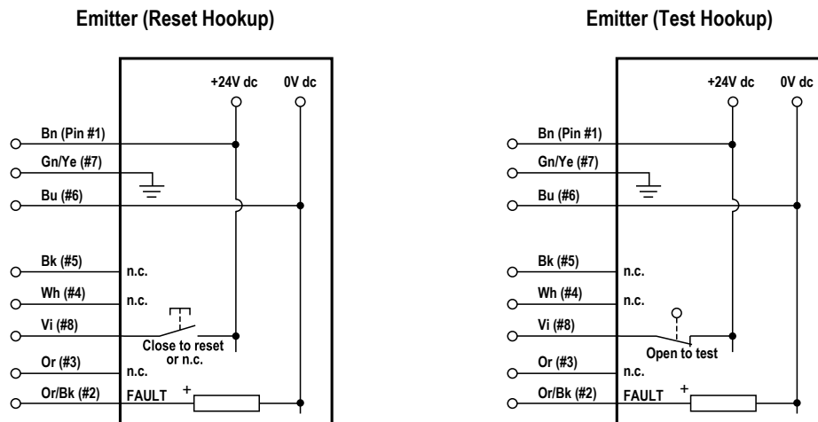
Figure 28. Emitter—Generic wiring
