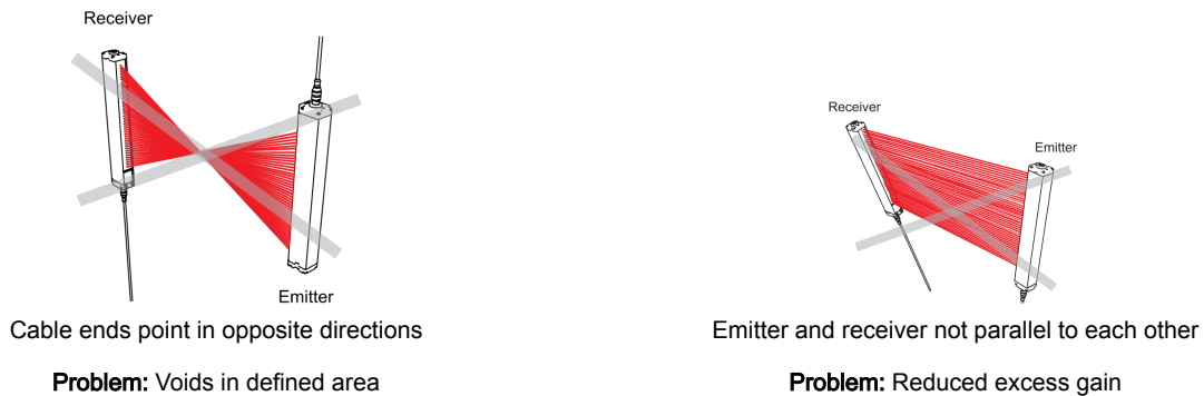
Figure 7. Examples of Incorrect Emitter/Receiver Orientation
