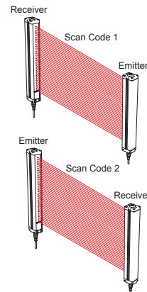
Figure 9. Two or three systems stacked (or alternate receiver/emitter positions)
