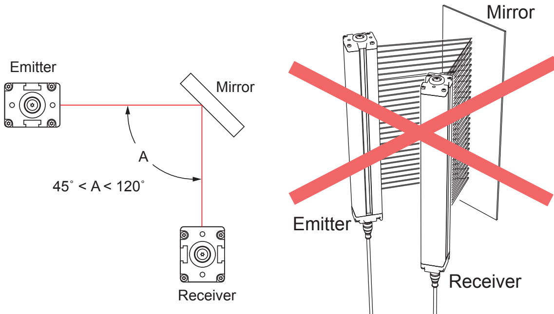
Figure 5. Using EZ-SCREEN LPM sensors in a retroreflective mode
