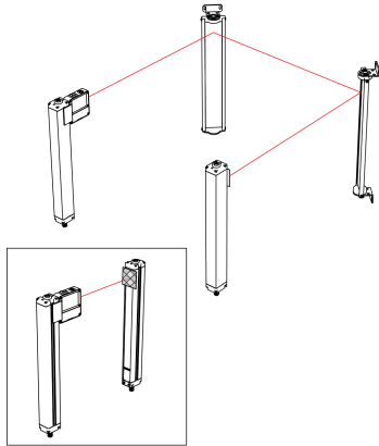
Figure 21. Optical alignment using the LAT-1
