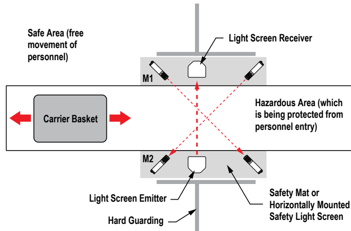
Figure 33. Horizontal photoelectric muting devices placed at different heights
