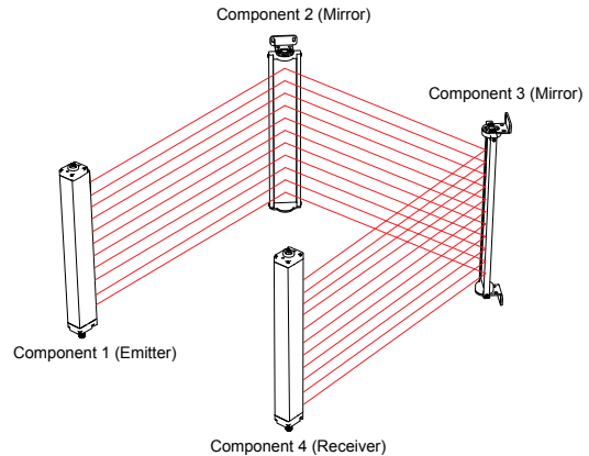
Figure 22. Corner Mirror Alignment
