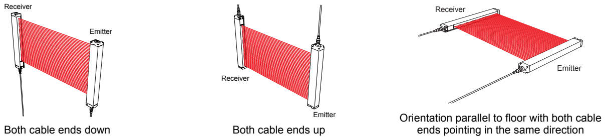
Figure 7. Examples of Incorrect Emitter/Receiver Orientation
