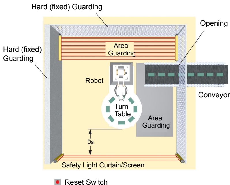
Figure 3. An example of supplemental safeguarding
