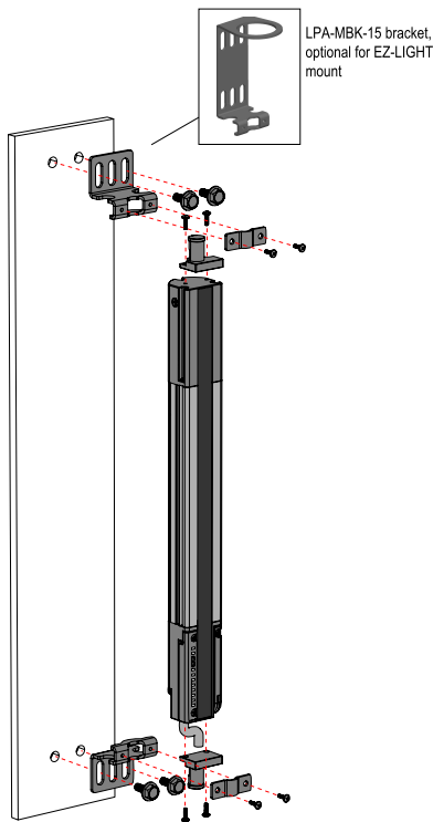
Figure 12. End-Mount Brackets
