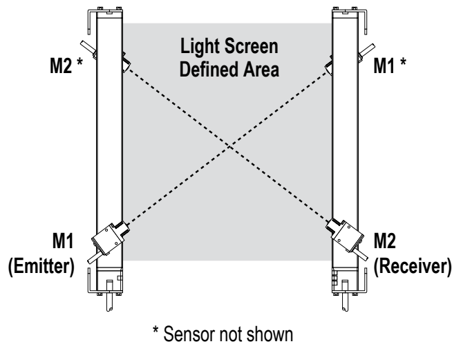
Figure 34. Photoelectric muting devices placed diagonally
