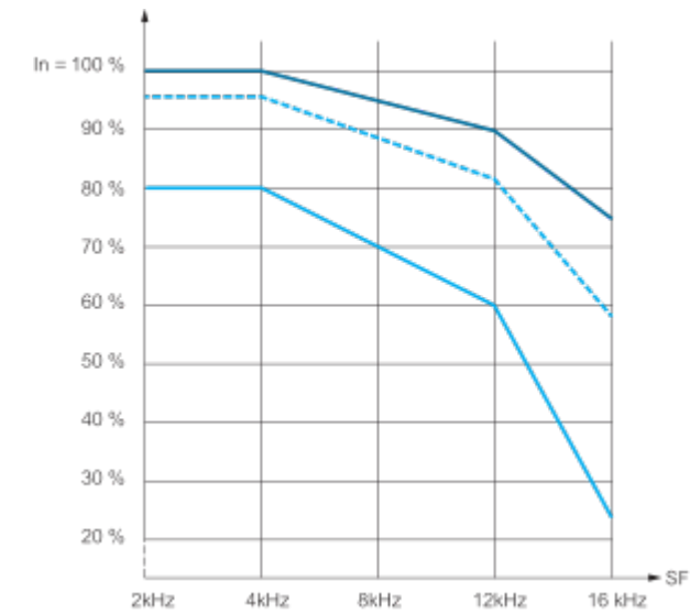
— 40 °C (104 °F) - Mounting type B - - - 50 °C (122 °F) - Mounting type B — 60 °C (140 °F) - Mounting type B In : Nominal Drive Current SF : Switching Frequency
