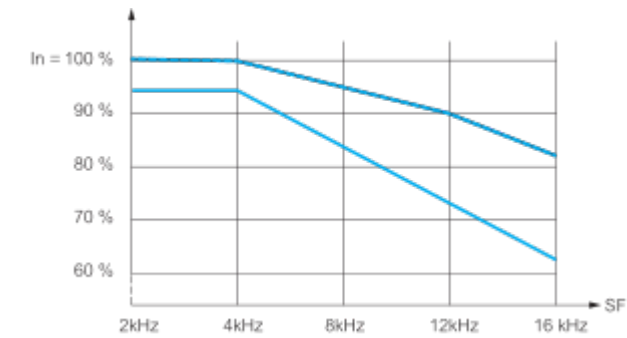
— 40 °C (104 °F) - Mounting type B - - - 50 °C (122 °F) - Mounting type B — 60 °C (140 °F) - Mounting type B In : Nominal Drive Current SF : Switching Frequency
