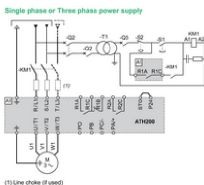
Control Block Wiring Diagram
