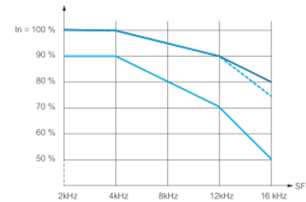
— 40 °C (104 °F) - Mounting type A - - - 50 °C (122 °F) - Mounting type A — 60 °C (140 °F) - Mounting type A In : Nominal Drive Current SF : Switching Frequency
