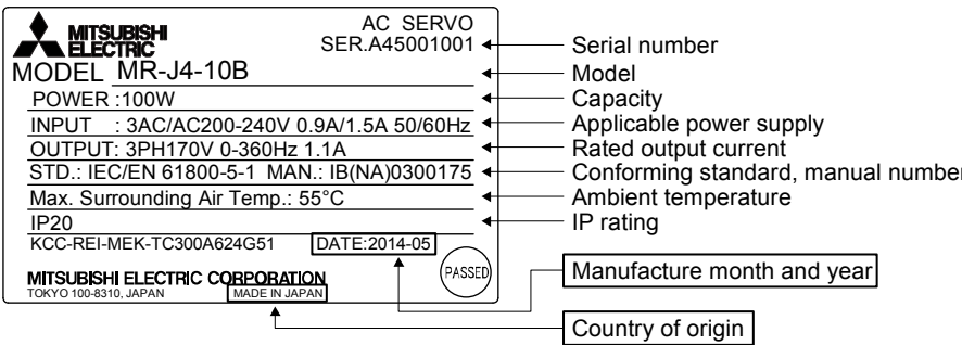
Fig. app. 3 Indication example on the rating plate
