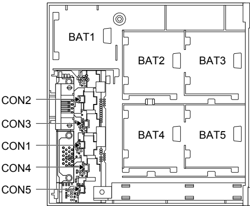
Parts identification
